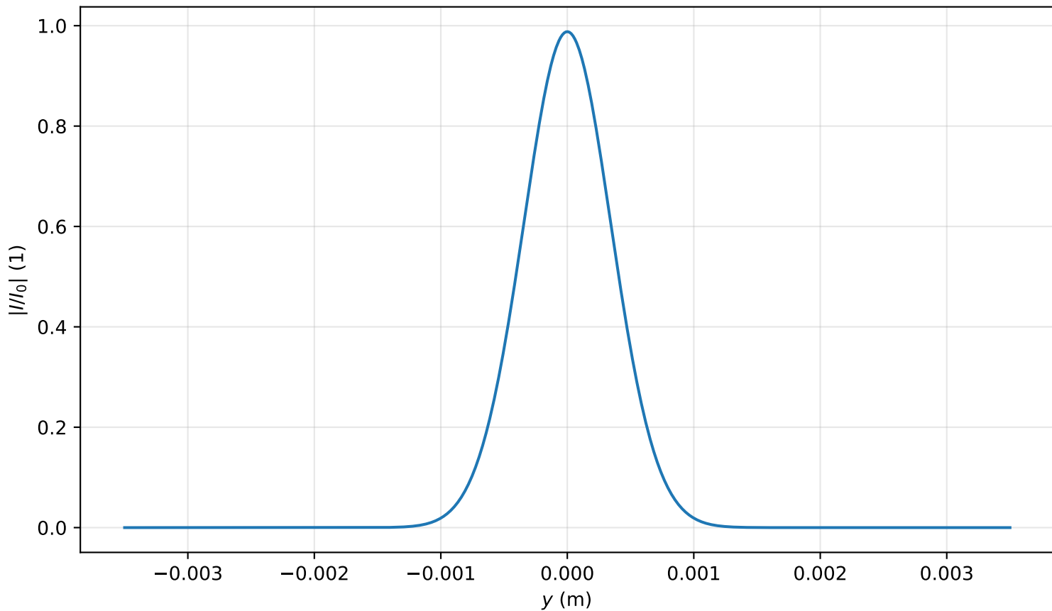
Intensity profile I(x=0, y, z=0.398)/I_0 , P_{in}=0.2P_{cr} , artificial time
